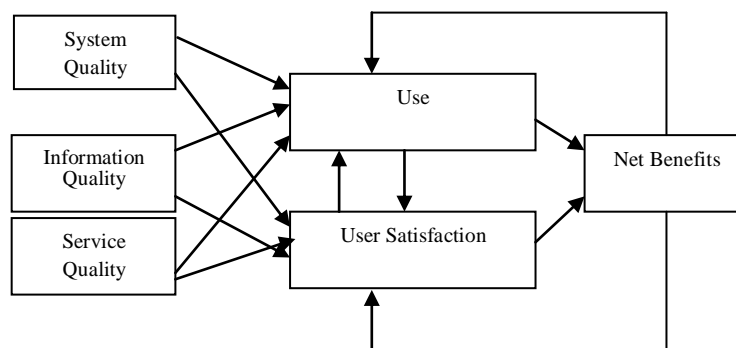
Figure 1: D&M model
